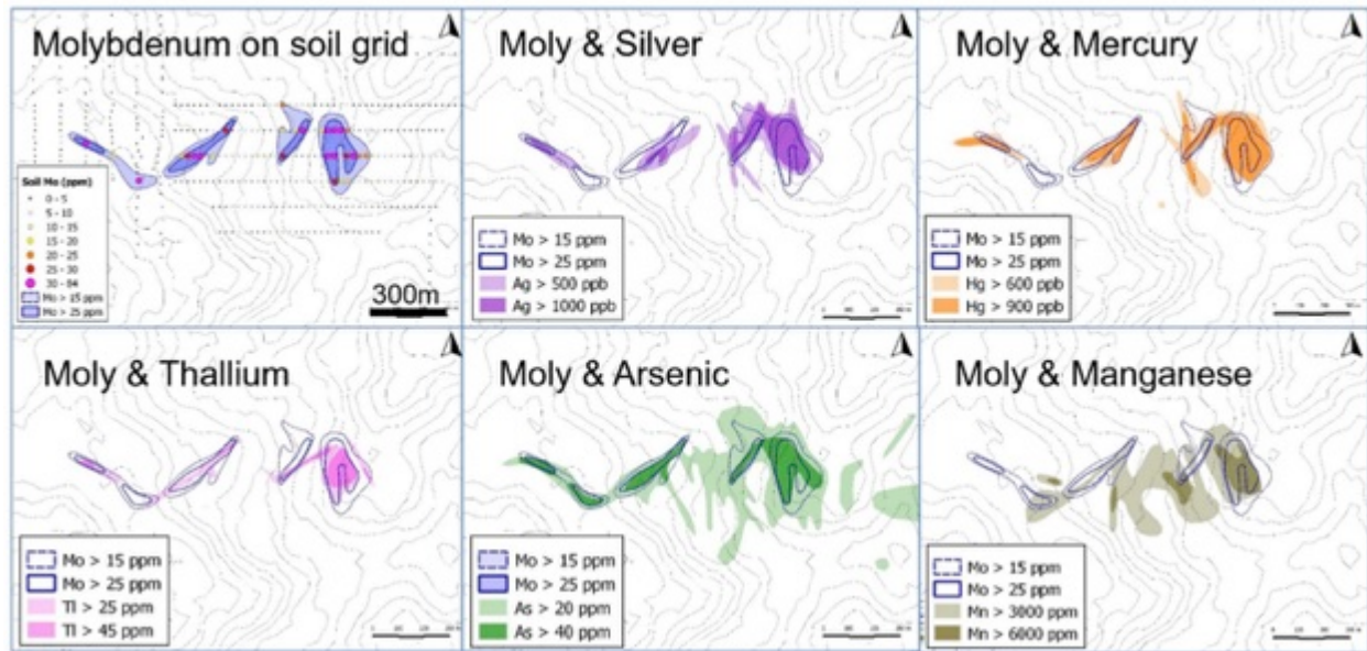
Figure 1. Summary of distribution of pathfinder elements in soil at Crunchy Hill.
