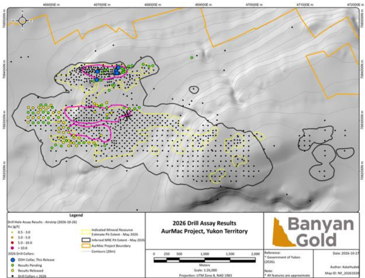
Figure 1: Plan map of AurMac, Yukon, Canada. Results for drillholes AX-26-904, -908, -909, -913, -915 and -921 are reported in Table 1. A plan map of Airstrip (Figure 2) and cross-sections (Figures 3 and 4) show the detailed distribution of drillholes in Airstrip and the geometry of high-grade mineralization.
