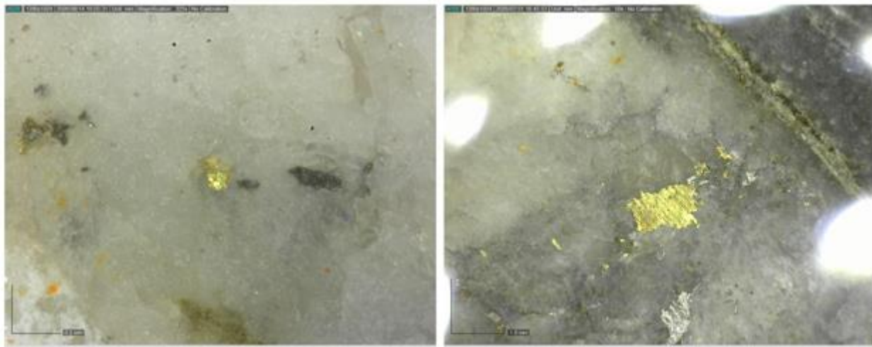
Figure 6: Visible gold in extensional quartz veins from: Left - hole AX-26-921, from 265.1 m – gold associated with bismuth sulphosalts and arsenopyrite in an extensional quartz vein. Right – hole AX-26-913, from 176.3 m – gold associated with arsenopyrite in an extensional quartz vein.
