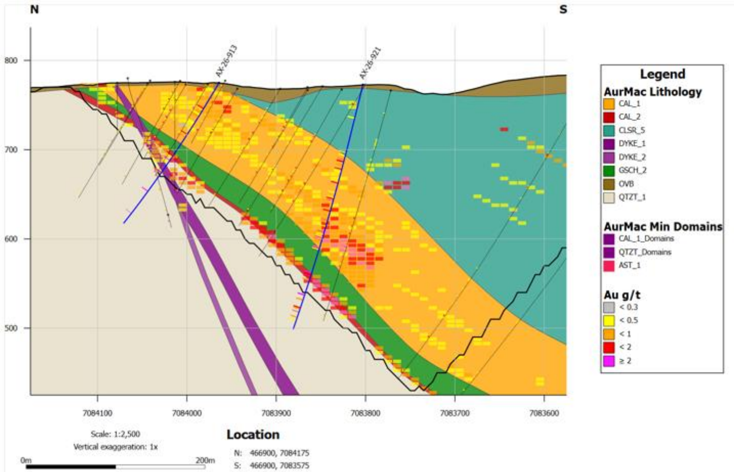
Figure 3: Cross-section 466900mE through Airstrip. Drillhole AX-26-921 highlights potential expansion of high-grade domains in the gap zone between Airstrip and Powerline. Additional down-dip drilling is planned to further test the extent of high-grade mineralization at depth within and just south of the conceptual pit boundary. The MRE block model is constrained by mineralized and lithological domains. Mineral Resource blocks are 10 m x 10 m x 5 m. Only blocks above the 0.30 g/t Au cut-off and within the US$3,500/oz Au conceptual pit shell are included in the MRE.
