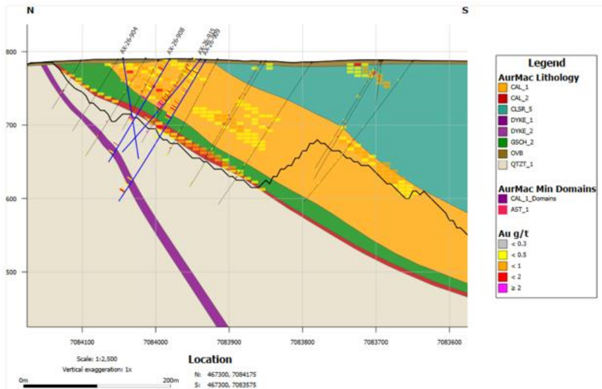
Figure 4: Cross-section 467300mE through the eastern end of Airstrip at AurMac. Drillholes in this release demonstrate potential for improvement in grade in mineralized domains in the eastern end of Airstrip. The MRE block model is constrained by mineralized and lithological domains. Mineral Resource blocks are 10 m x 10 m x 5 m. Only blocks above the 0.30 g/t Au cut-off and within the US$3,500/oz Au conceptual pit shell are included in the MRE.
