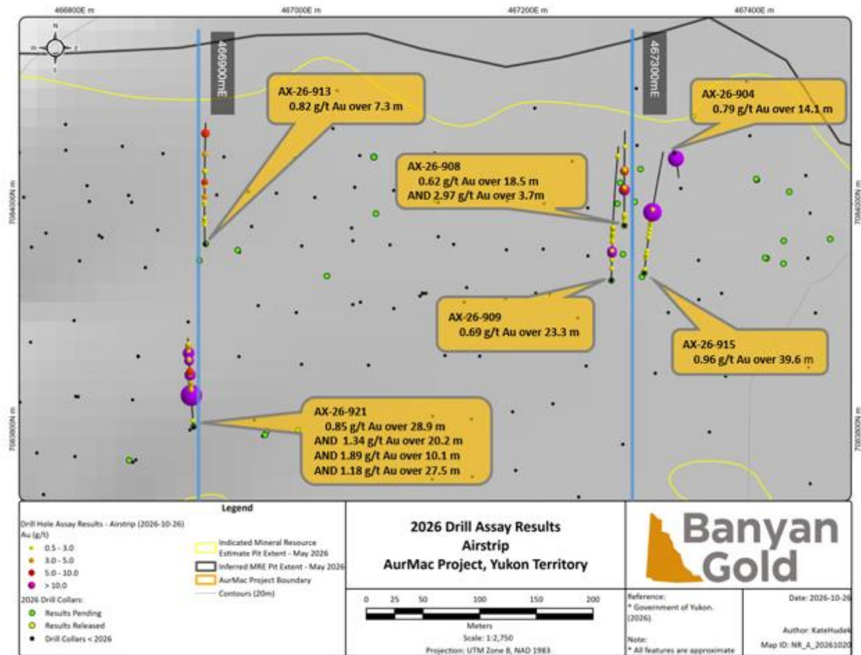
Figure 2: Plan map of Airstrip. Cross-sections are denoted by blue lines. Drillhole AX-26-921 in cross-section 466900mE (Figure 3) highlights the expansion potential for high-grade domains in the gap between the Airstrip and Powerline Deposits near the southern extent of the conceptual Mineral Resource Estimate (“MRE”) pit. Drillholes AX-26-904, -908, -909, and -915 in cross-section 467300mE (Figure 4) highlight the expansion potential for high-grade domains to the east in Airstrip.
