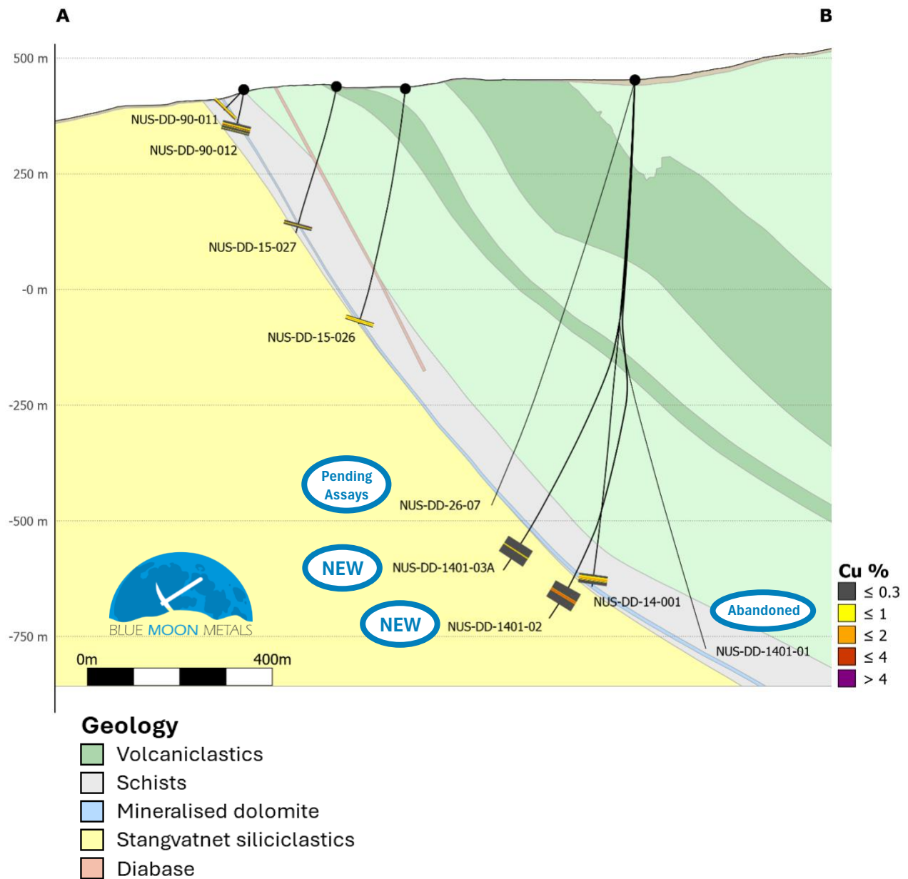
Figure 3, A cross section of the deep navigational drilling that continues in the West of Nussir's known mineralization.
