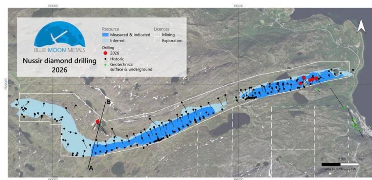
Figure 1, A plan view map displaying current drill hole locations across the Nussir project. Note the defined resource classification resulting from the 2025 NI 43-101 Technical Report by Adam Wheeler
