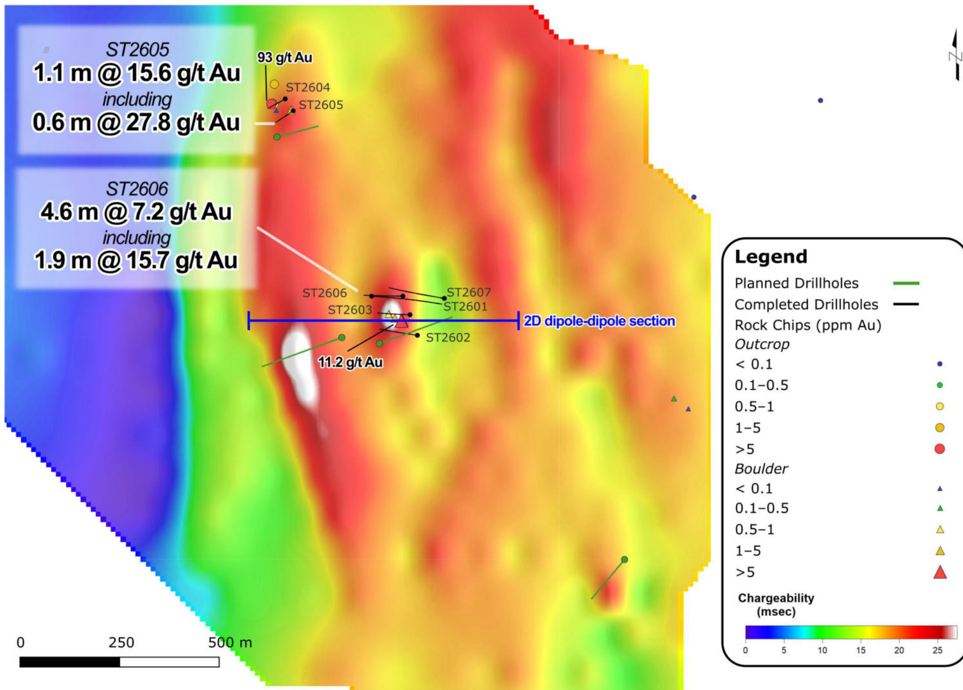
Figure 3: Plan view of gradient-array IP chargeability at the Stavaträsk project, showing maiden drill hole collars (ST2601 to ST2607) and planned collars for the second drill program.
