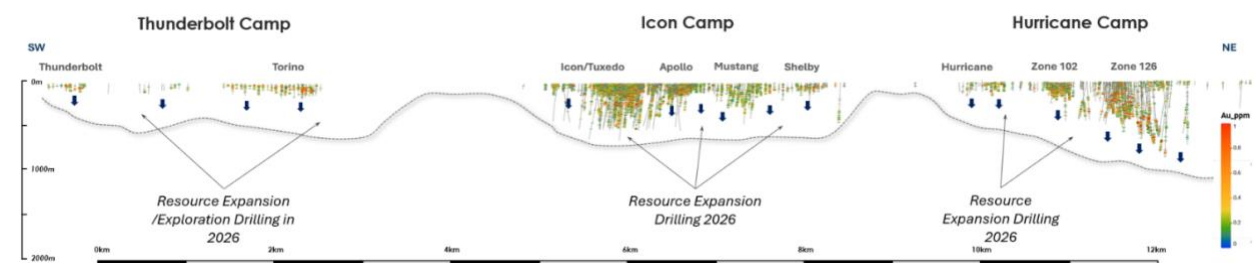
Figure 4: NE-SW oriented long section through the Glenburgh project showing distribution of drillholes and assays; and the emergence of three defined camps with almost contiguous mineralization. Thunderbolt camp has yet to be tested by Benz drilling.
